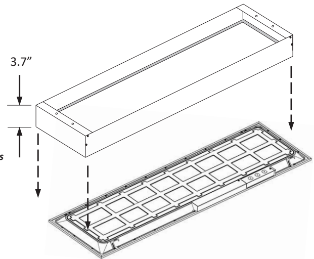
Surface Mounting Kits (10-SMKT-14)
