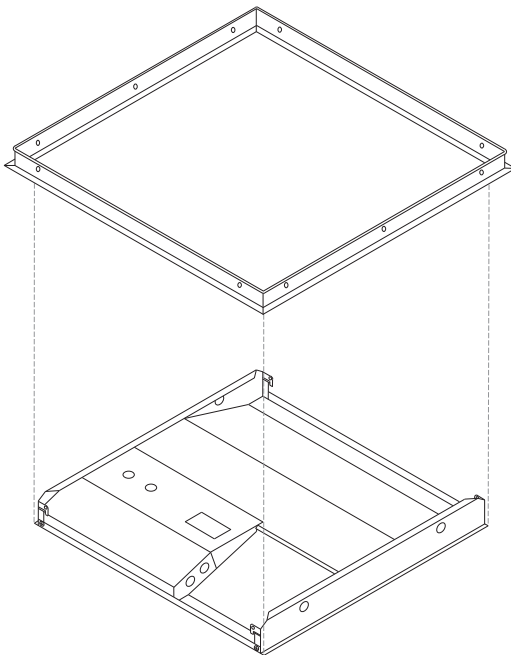
Flange Mount Kit (10-LEDPNL2x2-FK)
